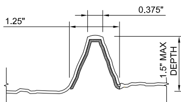
OVERLAP FORMLINER DETAIL
