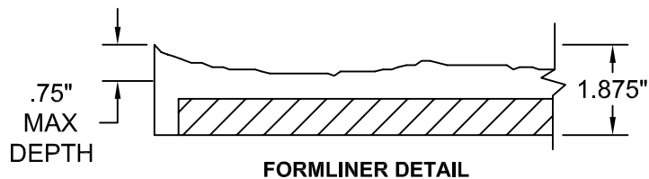
FORMLINER DETAIL
