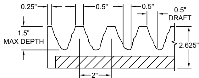
FORMLINER DETAIL
