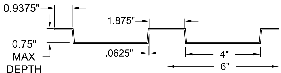
FORMLINER DETAIL
