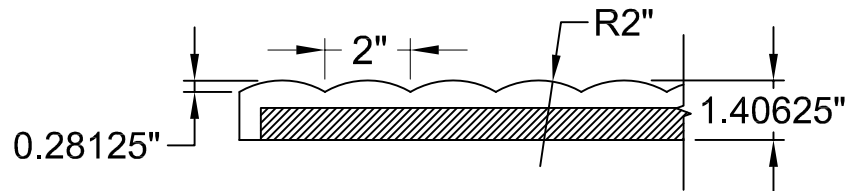
FORMLINER DETAIL
