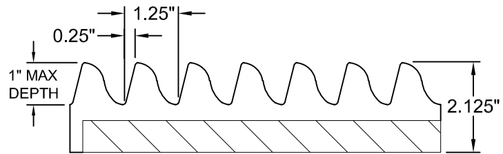
FORMLINER DETAIL
