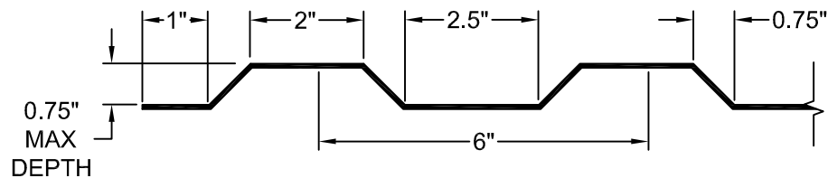
FORMLINER DETAIL
