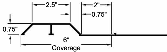
FORMLINER DETAIL
