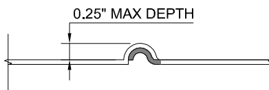
OVERLAP FORMLINER DETAIL
