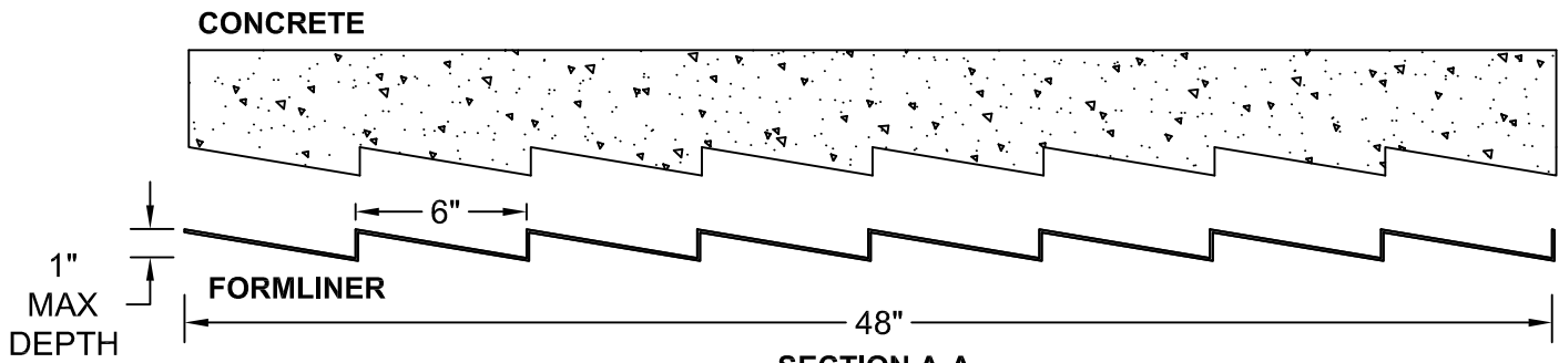
SECTION A-A FORMLINER DETAIL
