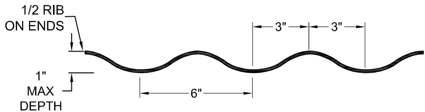
FORMLINER DETAIL
