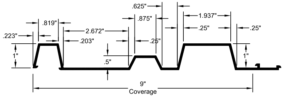
FORMLINER DETAIL
