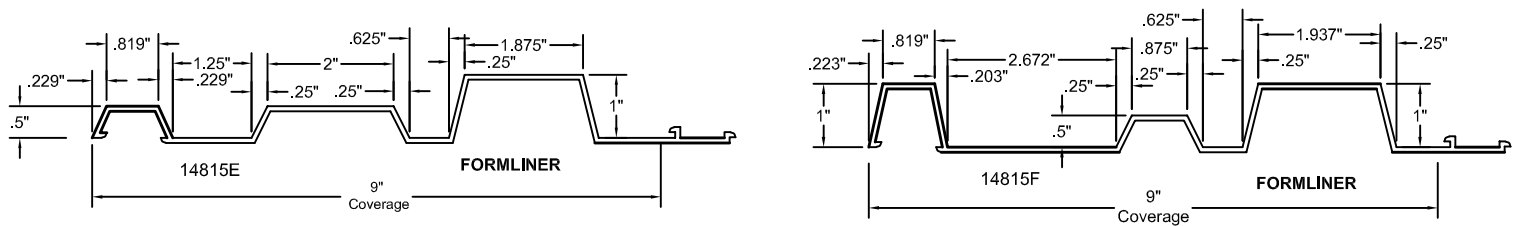
FORMLINER DETAIL
