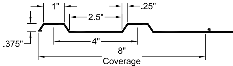
FORMLINER DETAIL
