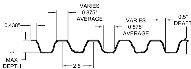
FORMLINER DETAIL
