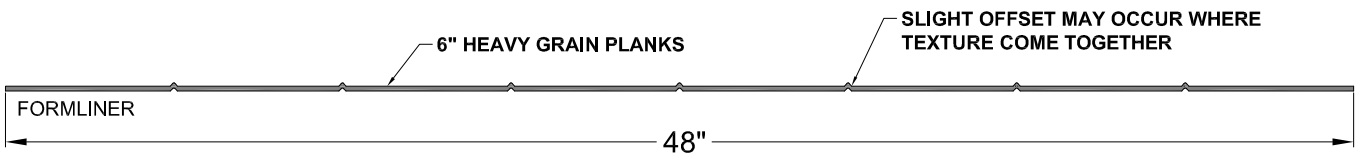
SECTION A-A FORMLINER DETAIL
