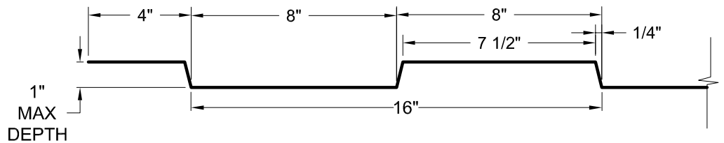
FORMLINER DETAIL
