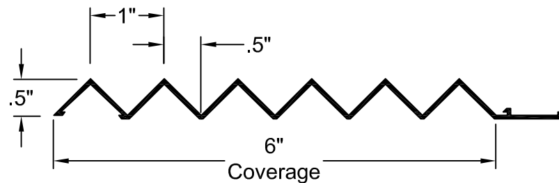
FORMLINER DETAIL
