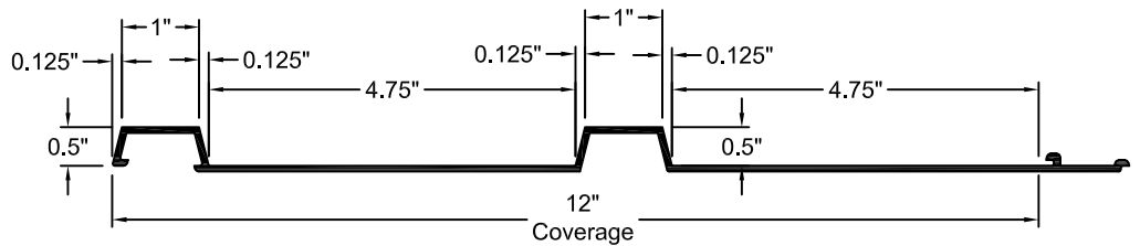
FORMLINER DETAIL
