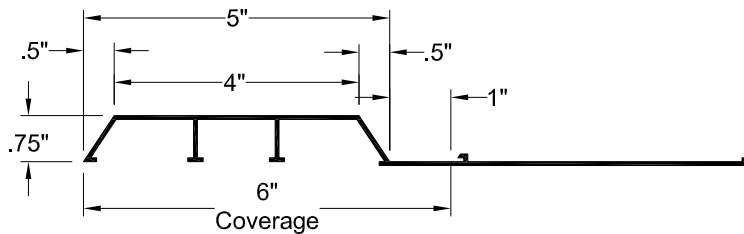
FORMLINER DETAIL
