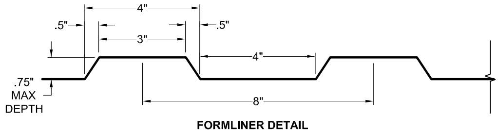
FORMLINER DETAIL
