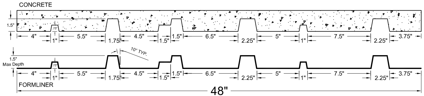
SECTION A-A FORMLINER DETAIL
