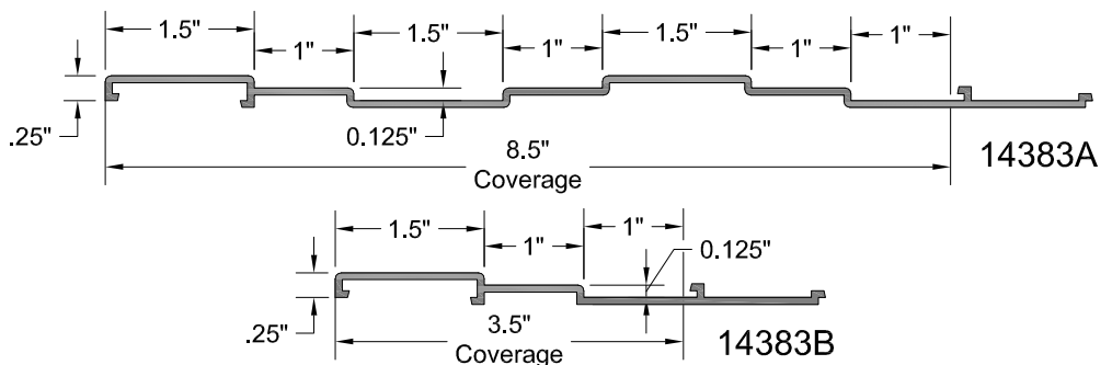
FORMLINER DETAIL
