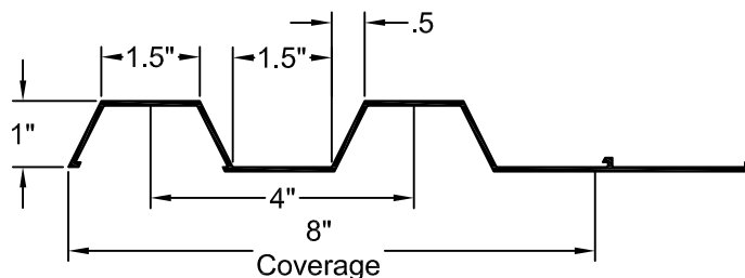
FORMLINER DETAIL
