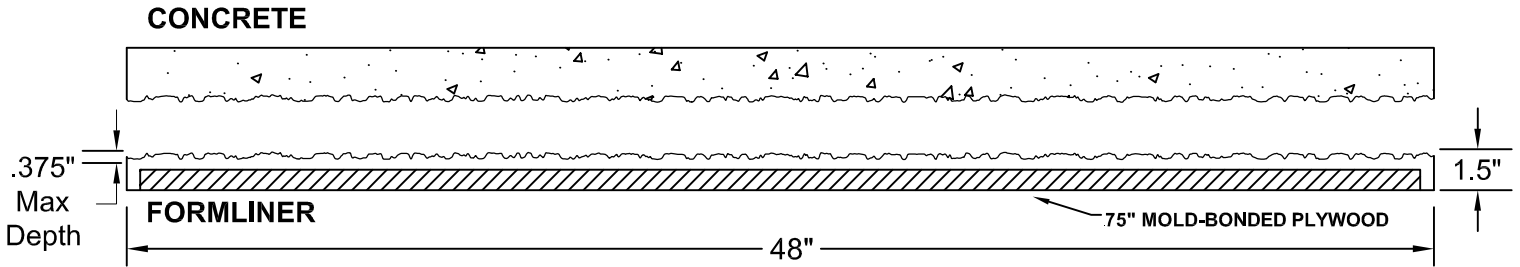
SECTION A-A FORMLINER DETAIL
