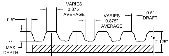
FORMLINER DETAIL
