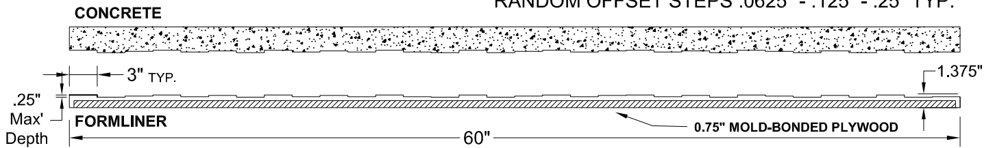
SECTION A-A FORMLINER DETAIL
