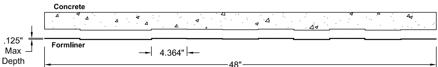
Section A-A FORMLINER DETAIL
