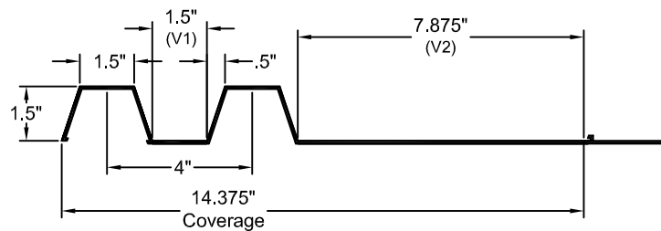
FORMLINER DETAIL
