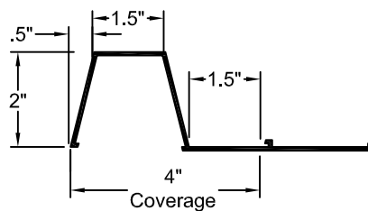
FORMLINER DETAIL
