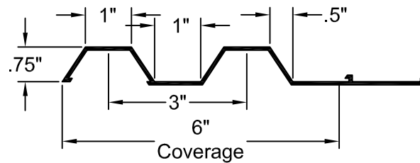
FORMLINER DETAIL
