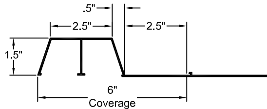
FORMLINER DETAIL
