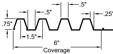
FORMLINER DETAIL
