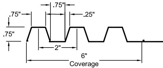
FORMLINER DETAIL
