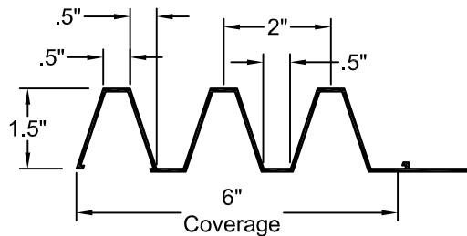
FORMLINER DETAIL
