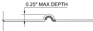
OVERLAP FORMLINER DETAIL
