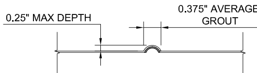
OVERLAP FORMLINER DETAIL
