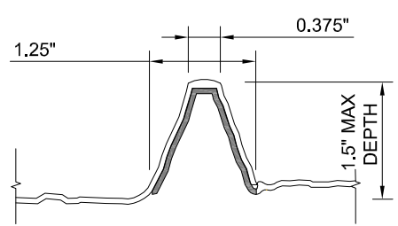
OVERLAP FORMLINER DETAIL
