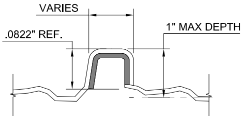
OVERLAP FORMLINER DETAIL
