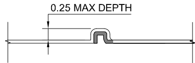
OVERLAP FORMLINER DETAIL
