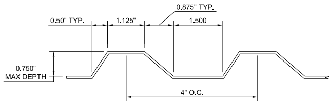
FORMLINER DETAIL
