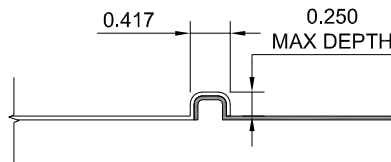
FORMLINER DETAIL
