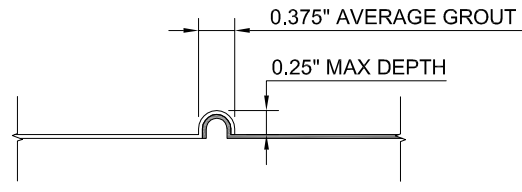
FORMLINER DETAIL
