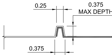
FORMLINER DETAIL
