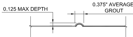
FORMLINER DETAIL
