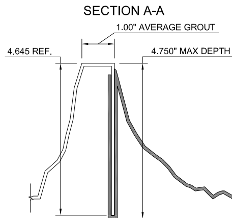
FORMLINER DETAIL
