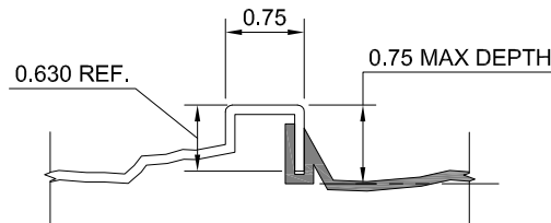
FORMLINER DETAIL
