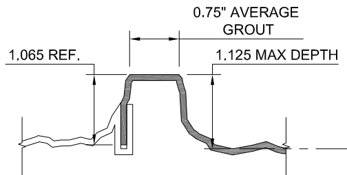
FORMLINER DETAIL
