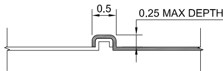
FORMLINER DETAIL
