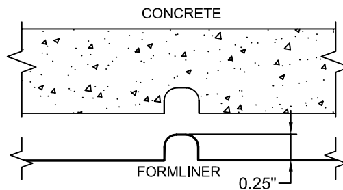
SECTION A-A FORMLINER DETAIL
